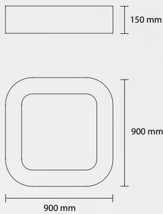
PL KUA 90 3 E27 42W ALO 1 LED 30W 2800LM 3000K
