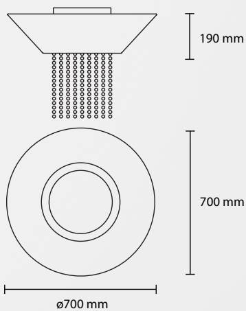
PL BROLLO 70 2 E27 42W ALO 1 LED 18W 1800LM 3000K
