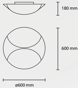
PLT SINUA 60 2 E27 42W ALO 1 LED 18W 1800LM 3000K
