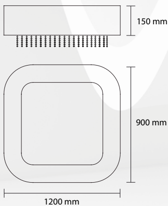
PL CRISTAL Q 120 3 E27 42W ALO 1 LED 30W 2800LM 3000K
